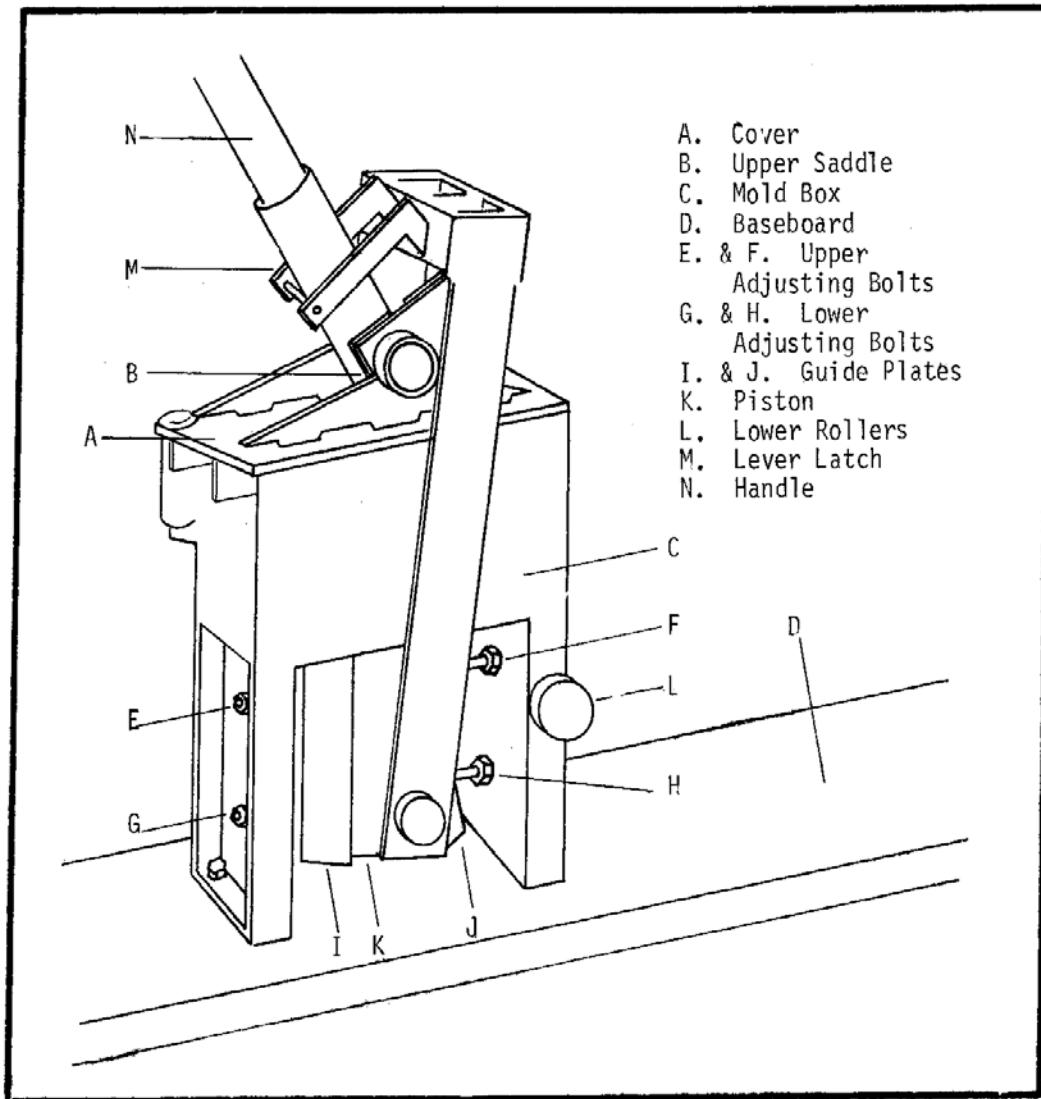
Fig. 1 - The CINVA-Ram Block Press and Its Parts
